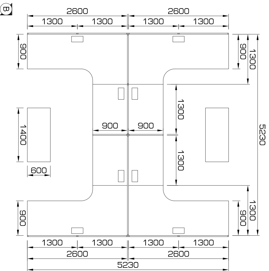
A PLAN VIEW SCALE 1:50
